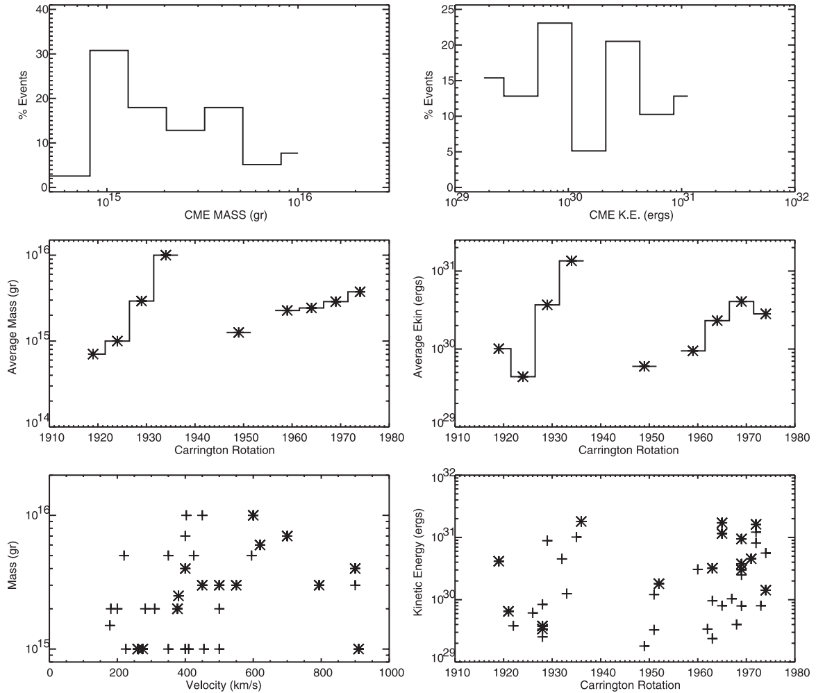
Fig. 4. Statistics for our flux-rope CME sample. Top left: Histogram of CME masses. Top right: Histogram of CME kinetic energies. CME mass as a function of Carrington rotation ( middle left ) and CME kinetic energy as a function of Carrington rotation ( middle right ). The bins are averages over 5 rotations. Scatterplot of CME mass versus front speed ( bottom left ) and CME kinetic energy versus Carrington rotation ( bottom right ). The stars correspond to the events associated with eruptive prominences.
