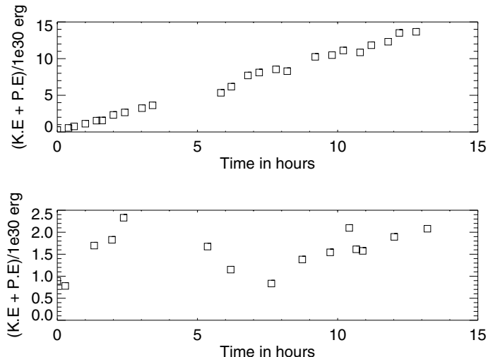
Fig. 1. The mechanical (i.e., kinetic + potential) energy for two representative CMEs plotted as a function of time from initiation. The mechanical energy for the CME on 2000/03/22 ( upper panel ) increases linearly with time, implying that there is a constant driving power on the CME as it propagates outwards. Such CMEs are included in category A (Table 1). The mechanical energy for the CME on 1998/08/13 ( lower panel ) shows no such trend. Such CMEs are included in category B (Table 2).
