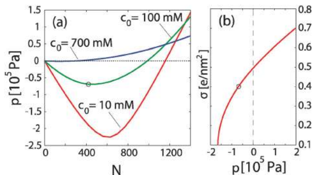
Fig. 8 Panel (a): Osmotic pressure acting on the viral capsid as a function of the number of monomers. Panel (b): Osmotic pressure for fixed number of monomers N = 420 , c_0 = 100 mM [the point denoted by a circle in panel (a)] as a function of the capsid charge density, \sigma . The capsid is assumed to be infinitely thin, with a radius of R = 12 nm. Other parameters of the calculation are the same as in Fig. 4 (adapted from ref. 114).
