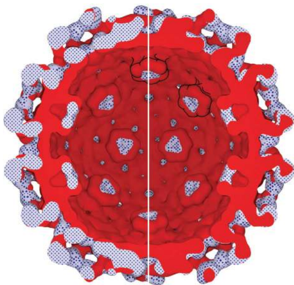
Fig. 5 One half of the cucumber mosaic (ssRNA) virus capsid (strain FNY). The image was constructed from RCSB Protein Databank entry 1F15 in the same manner as the one panel (c) of Fig. 2. One can observe “buttons” of positive charge density.
