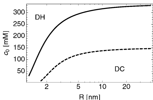
Fig. 9 The lines separating the positive (above) and negative (below) values of the total free energy of a model bacteriophage with \rho = -0.7 e_0 per \text{nm}^3 , obtained in the dressed counterion approximation. Above the lines the DH term dominates, whereas below the lines the DC term takes over. The bacteriophage is assumed to be in a bathing solution that contains 1 mM of \nu -valent salt, in addition to c_0 of monovalent salt. Full line for \nu = 4 and dashed for \nu = 2 .
