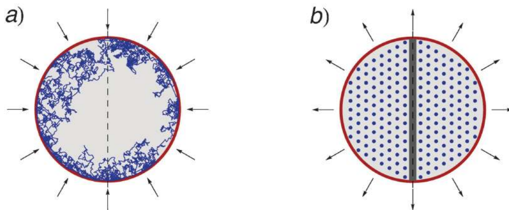
Fig. 7 Pressures sketch for an ssRNA [Panel (a)] vs. dsDNA virus [Panel (b)]. Genome is shown in blue, capsid in red, arrows indicate the direction of pressure. Cross section through the capsid. In the ssRNA case the genome is disordered but shows a distinct boundary layer close to the inner surface of the virus with a depleted region in the middle. In the dsDNA case the genome density within the capsid is (almost) uniform, showing pronounced orientational and positional ordering.
