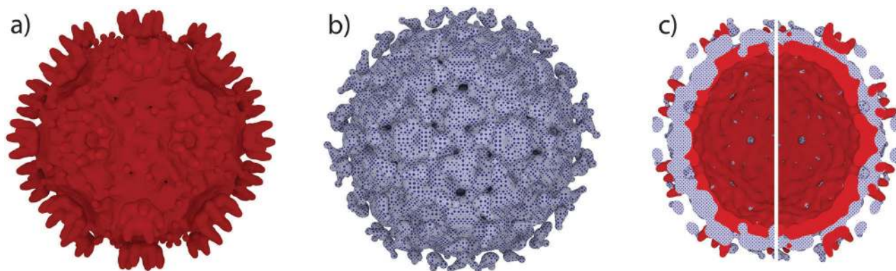
Fig. 2 The calculated representation of the charge distribution on the capsid of cowpea chlorotic mottle (ssRNA) virus as explained in the text, based on the 1CWP entry in the RCSB Protein Data Bank: (a) The isosurface of positive charge (single color pigment). (b) The isosurface of negative charge (dotted pattern). (c) The combined isosurfaces of positive and negative charges shown in the capsid cut in half so that its interior is seen. On the left-hand side of the image in panel (c) (the left of the white vertical line), the (cut) isosurface of negative charge (dotted pattern) is translated infinitesimally closer to the viewer, while it is the opposite on the right-hand side of the image.
