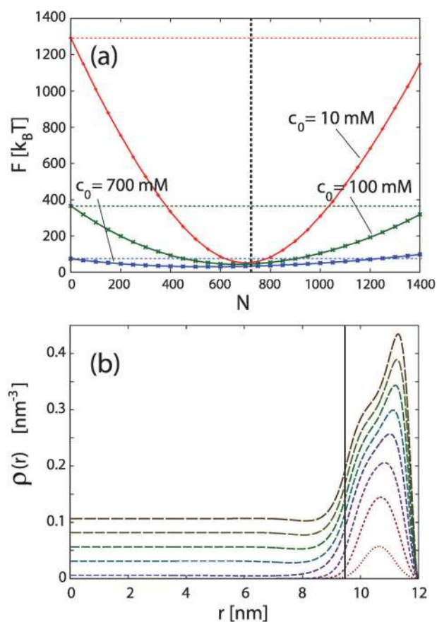
Fig. 6 Panel (a): The free energy of the capsid–ssRNA complex as a function of the total number of ssRNA bases. The capsid radius is R = 12 nm. The capsid charge, comprising of 724 elementary positive charges, is distributed in a spherical shell of 2.5 nm thickness. Panel (b): The ssRNA density profiles for N = 100, 300, 500, 700, 900, 1100, 1300, and 1500 . A vertical line at r = 9.5 nm indicates the position of the N-termini of the capsid proteins, i.e. the interior surface of the charged protein shell.
