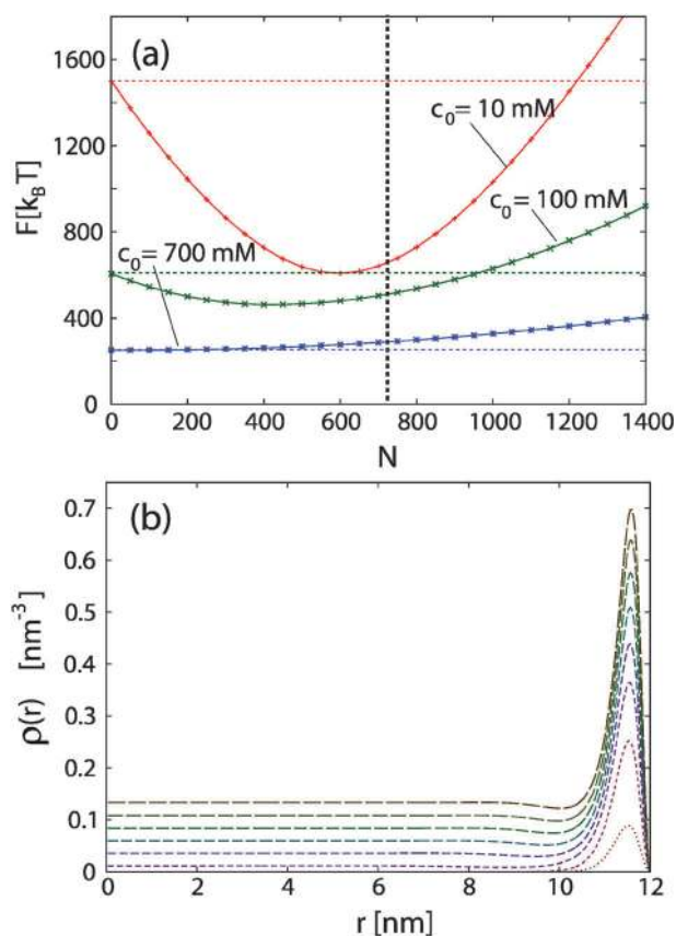
Fig. 4 Panel (a): The free energies of the capsid–ssRNA complexes as a function of the number of RNA bases and for three different monovalent salt concentration, as indicated. The free energy of the empty capsid is obtained when N = 0 . Panel (b): The ssRNA ( a = 0.5 nm) concentration profile in a capsid of radius R = 12 nm and surface charge density \sigma = 0.4 e_0 per \text{nm}^2 for c_0 = 100 mM. The curves displayed correspond to N = 100, 300, 500, 700, 900, 1100, 1300, and 1500 bases. The lines are styled so that the length of their dashes is proportional to N . See ref. 114 for details.
