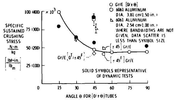
(a) Graphite/epoxy tubes.
