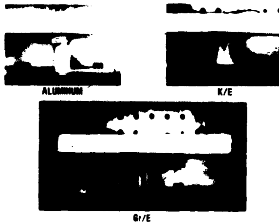
Figure 8. - Dynamically crushed aluminum, Kevlar/epoxy and graphite/epoxy tubes.
