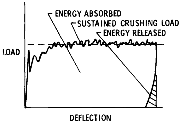
Figure 3. - Typical load-deflection curve of composite tube.
