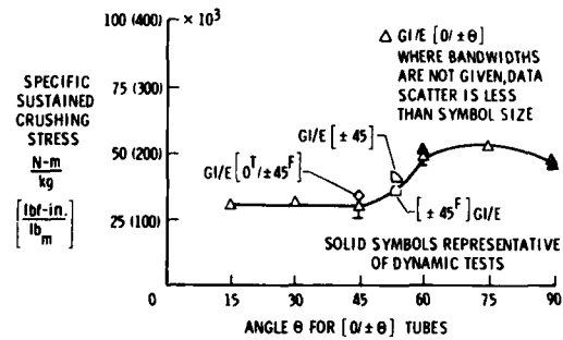
(c) Glass/epoxy tubes.
