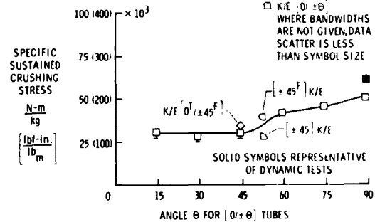
(b) Kevlar/epoxy tubes.
