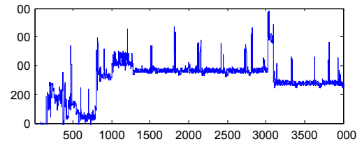
Figure 10: Measured GPS power profile.
