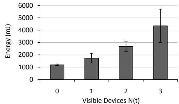
Figure 7: Bluetooth energy usage variation.
