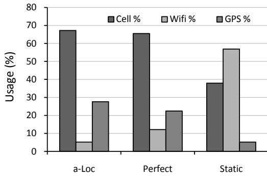
Figure 18: Modalities used by a-Loc and other approaches.
