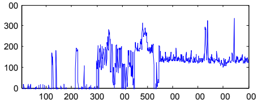
Figure 8: Bluetooth power usage during scan.
