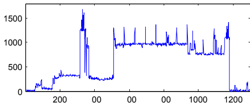
Figure 5: Measured power profile for WiFi.
