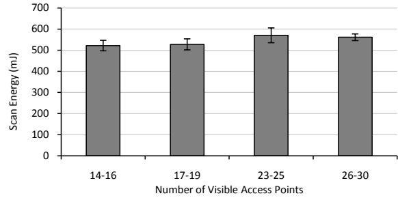
Figure 6: Energy usage for WiFi.
