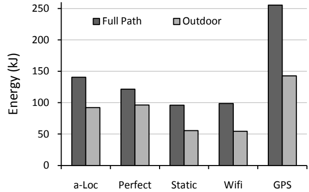
Figure 17: Energy consumption in San Diego experiments.
