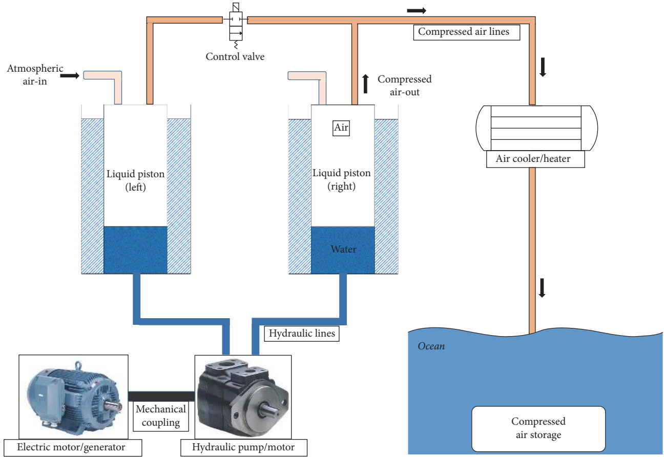
FIGURE 4: Schematic of a liquid piston based isothermal OCAES system.
