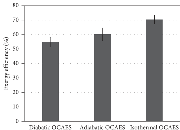
FIGURE 8: Overall exergy efficiency of different types of OCAES.
