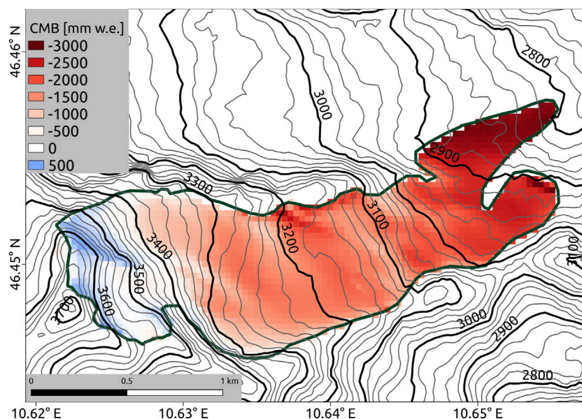
FIGURE 7 Spatially resolved simulated mean annual climatic mass balance (CMB), 2013–2017 [mm w.e.] for present climate.
