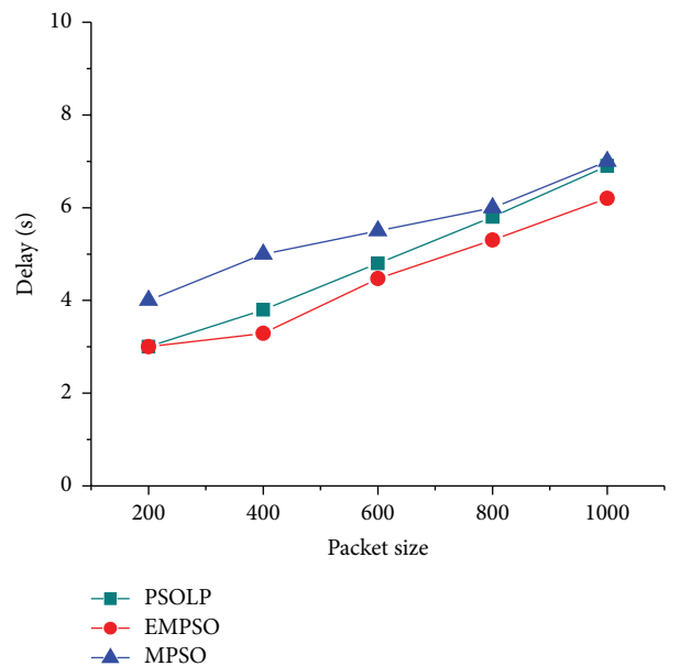
FIGURE 6: Delay versus packet size.
