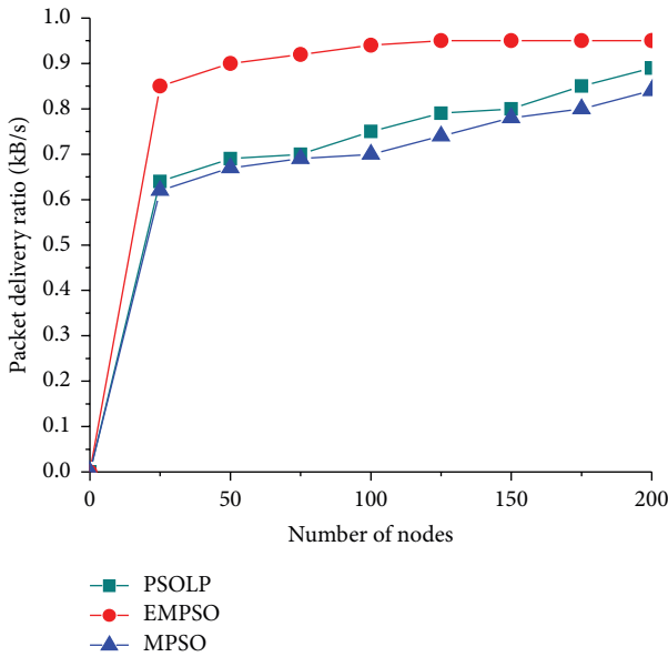
FIGURE 3: Packet delivery ratio versus number of nodes.
