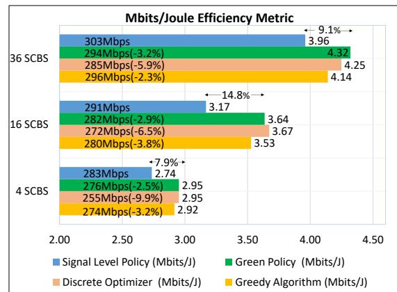
Fig. 8: Mbits/J Energy Efficiency Metric
