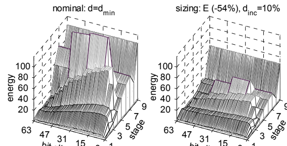
Fig. 6. Energy distribution, adder, WL = 32.
