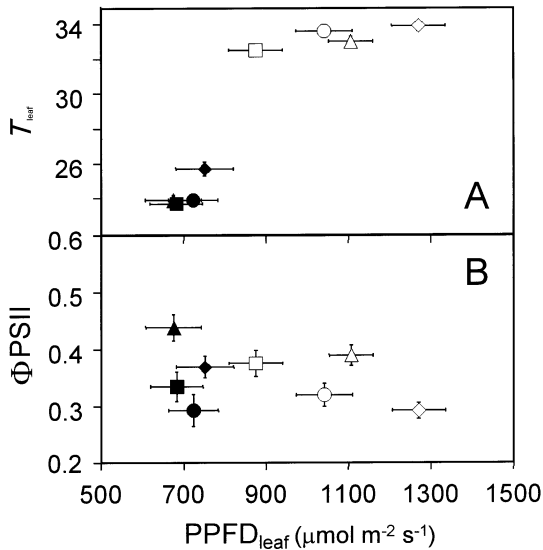
Figure 2. Mean values ( \pm SE) of (A) leaf temperature ( T_{leaf} ; n = 85 ) and (B) quantum yield of noncyclic electron transport ( \Phi_{PSII} ; n = 45-75 ) versus incident photon flux density ( PPFD_{leaf} ) at midday in current-year leaves of Quercus coccifera (●, ○), Q. ilex (■, □), Pinus halepensis (▲, △) and Juniperus phoenicea (◆, ◇) in summer 1996 (solid symbols) and 1997 (open symbols).
