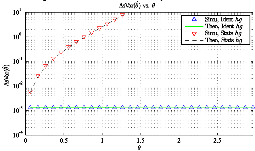
Figure 5-3: \text{AsVar}(\hat{\theta}) for Identical Constant and Statistical Gain Channels versus \theta .
