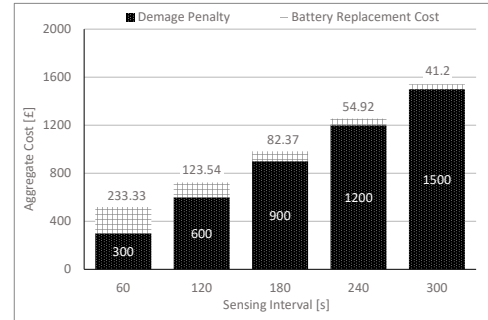
Fig. 8. Aggregate cost summarizing damage penalty and battery replacement cost when C_u = \text{£}10 , R_p = 30/\text{min}
