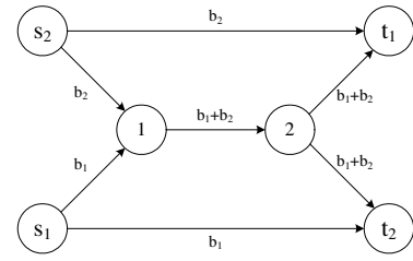
Fig. 1. The wireline butterfly network. Each link is with unit capacity. Two unicast sessions exist. s_i and t_i are source and receiver of session \tilde{u}_i , i = 1, 2 .
