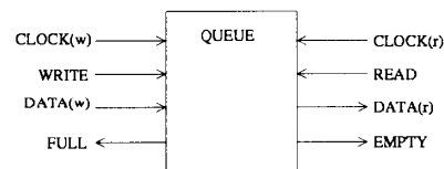
Figure 2. Queue structure
