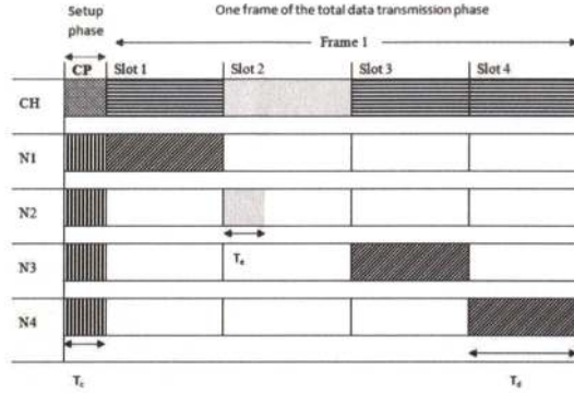
Fig. 3: Timing diagram of EA-TDMA protocol
