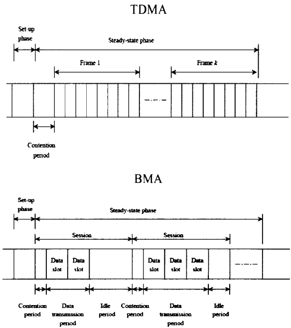
Fig. 1: Single round for TDMA and BMA protocol [8].
