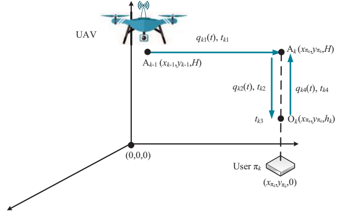
Fig. 2. Fly-hover-communicate protocol.
