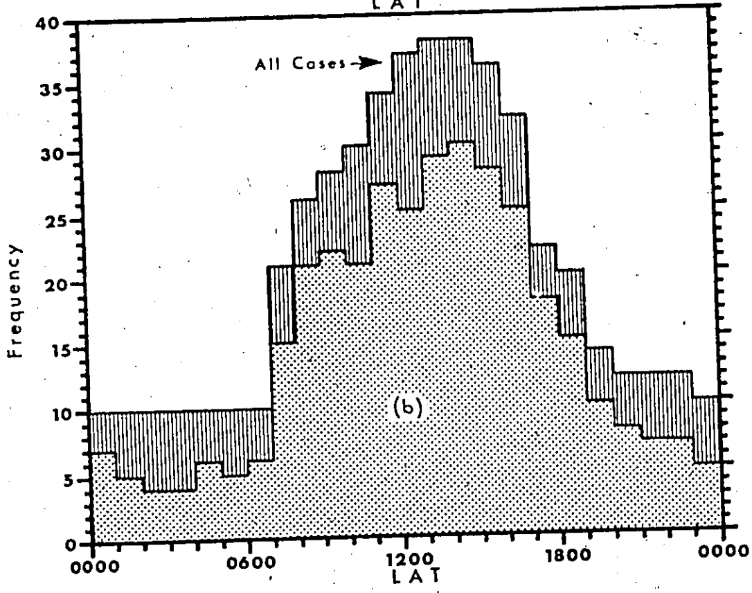
Figure 4.7. Frequency of observed boundary layer cases, (a) from wind profiles, and (b) from temperature profiles. Vertical hatching shows the difference between all cases observed and boundary layer cases.
