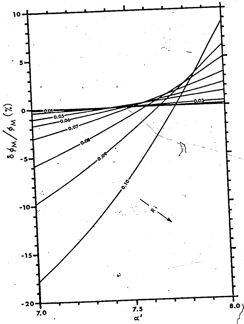
Figure 4.14. Relative error in \phi_M as a function of \alpha' and Ri .
