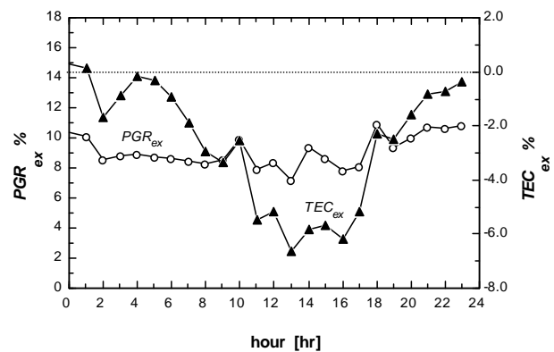
Figure 8. Variation of gas turbine exergetic PGR_{ex} and TE-C_{ex} during 18 th August operation.
