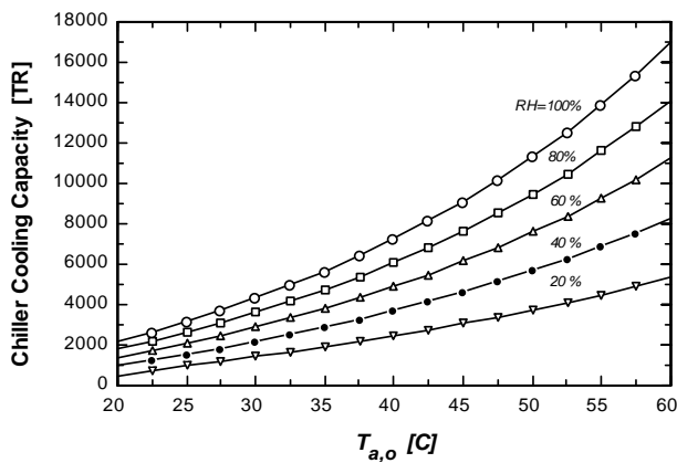
Figure 5. Dependence of chiller cooling capacity on the climatic conditions.
