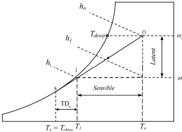
Figure 3. Moist air cooling process before GT compressor intake.
