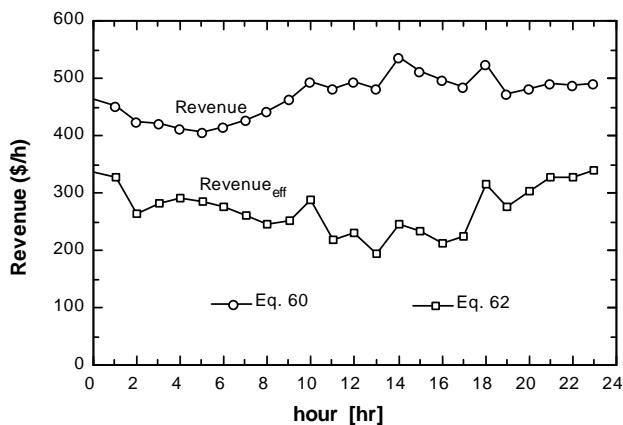
Figure 10. Effect of irreversibility on the revenue, C_{els} = 0.07 $/kWh.
