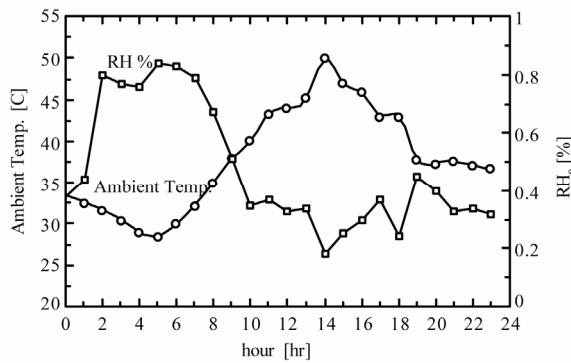
Figure 4. Ambient temperature variation and RH for 18 th of August 2010 of Yanbu Industrial City.
