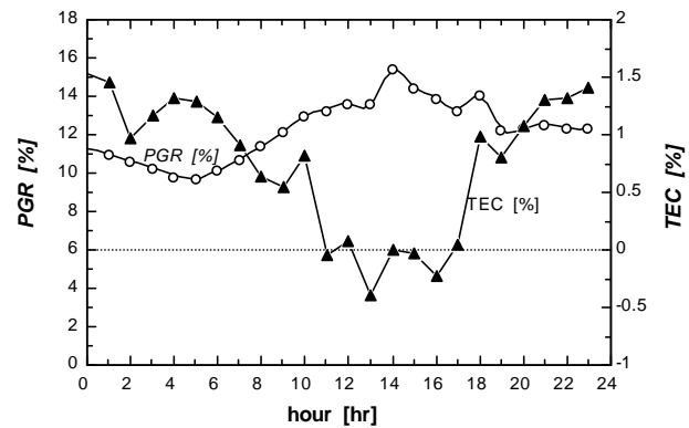
Figure 7. Variation of gas turbine PGR and TEC during 18 th August operation.
