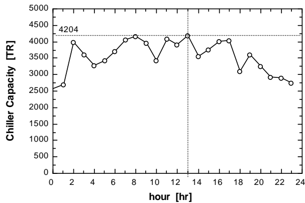
Figure 6. Chiller capacity variation with the climatic conditions of the selected design day.
