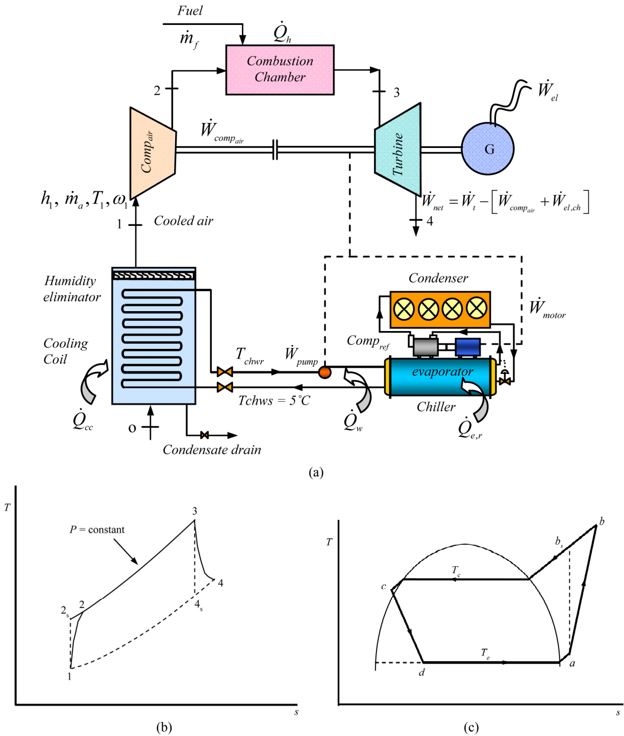
Figure 1. (a) Simple open type gas turbine with a chilled air-cooling unit; (b) T-s diagram of an open type gas turbine cycle; (c) T-s diagram for a refrigeration machine.
