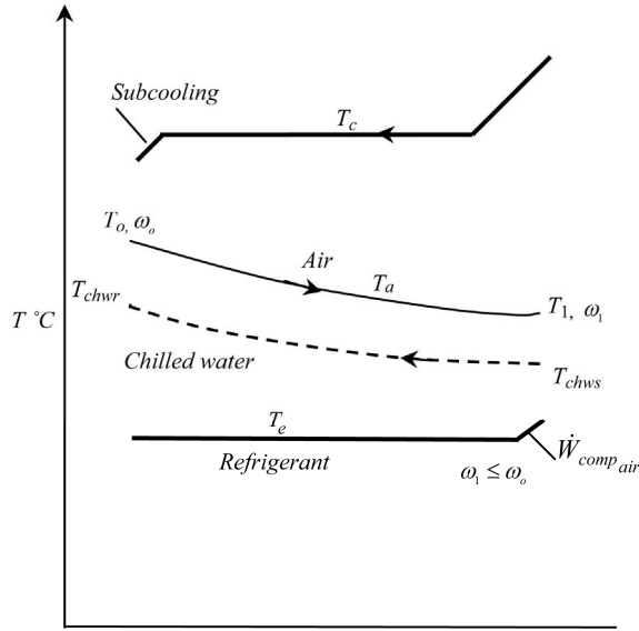
Figure 2. Temperature levels for the three working fluids, not to scale.
