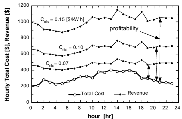
Figure 9. Variation of hourly total cost and excess revenue at different electricity selling rate.
