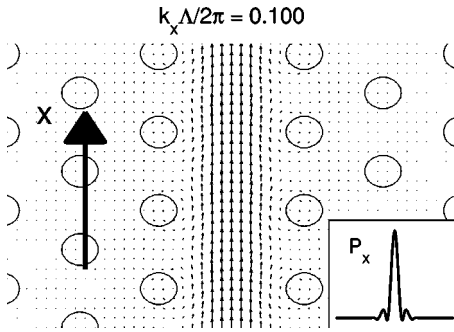
FIG. 5. The real part of the complex Poynting vector \mathbf{P} = \mathbf{E} \times \mathbf{H}^* for a Bloch mode, where the x component of the Bloch wave vector k_x is given by k_x \Lambda / 2 \pi = 0.100 . The inset shows an example of the x component of the Poynting vector across the waveguide.
