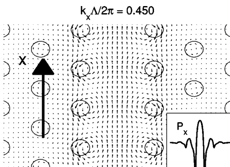
FIG. 6. The real part of the complex Poynting vector \mathbf{P} = \mathbf{E} \times \mathbf{H}^* for a Bloch mode, where the x component of the Bloch wave vector k_x is given by k_x \Lambda / 2 \pi = 0.450 . The inset shows an example of the x component of the Poynting vector across the waveguide.
