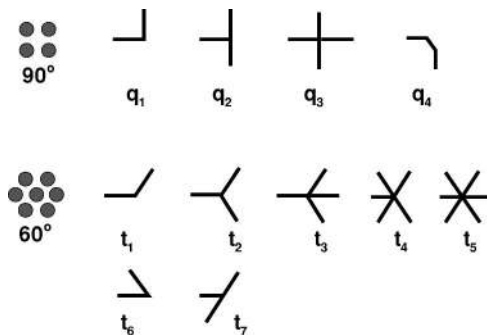
FIG. 11. Quadratic (90° symmetry) and triangular (60° symmetry) lattice crystals with some of the most obvious configurations of waveguide connections (branching points) for the redistribution of energy.
