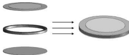
FIG. 1. Schematic diagram of a piezoelectric drum transducer.
