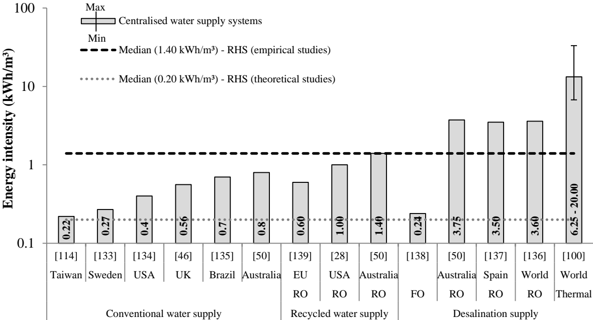
Fig. 1. Energy intensity comparison between centralised water supply systems and RHS [28,46,50,100,114,133–139].
