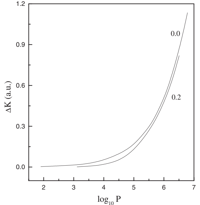
Fig. 2. Variation of change in kinetic energy ( \Delta K in a.u.) with logarithm of pressure at different screening.
