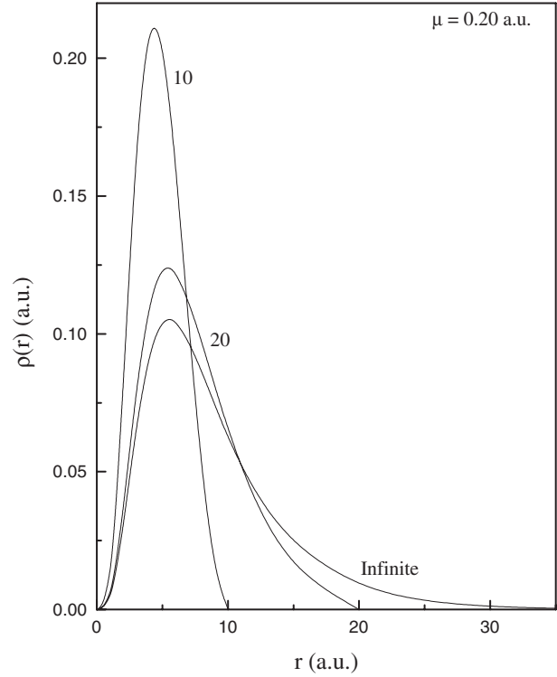
Fig. 7. Plot of charge density at different confinement with \mu = 0.2 a.u.
