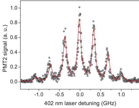
FIG. 4. (Color online) Fluorescence emission of trapped ^{232}\text{Th}^+ ions resulting from two-photon laser excitation registered with a broadband photomultiplier (300 to 650 nm). The peaks arise from excitation with different longitudinal modes of the Ti:sapphire laser. The solid line is a fit to equidistant Lorentzian lines under a Gaussian envelope.
