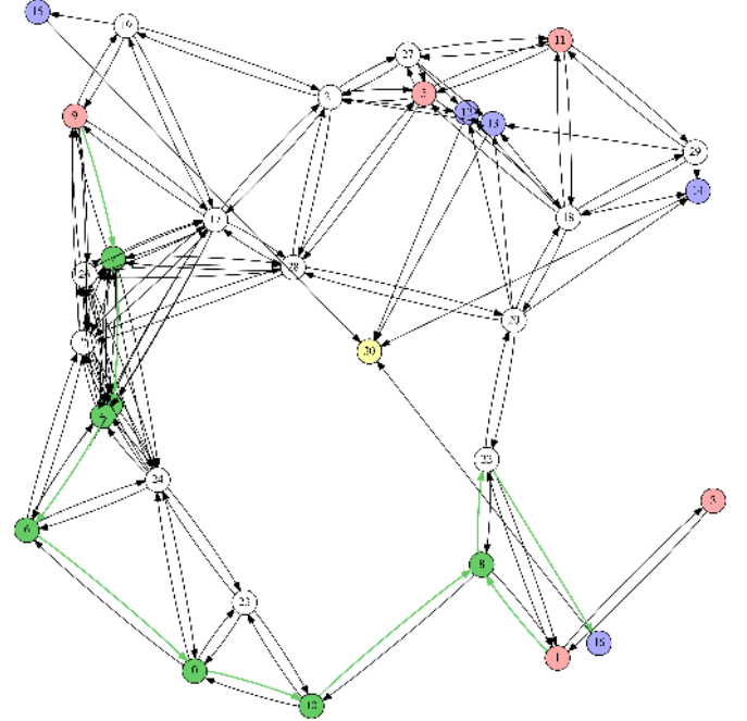
Fig. 7: An example routing solution for 1K with 30 nodes. Used links and aggregating nodes are shown in green.
