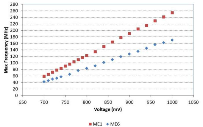
Fig. 8 Voltage and frequency.
