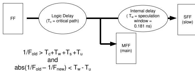
Fig. 6. Timing requirements
