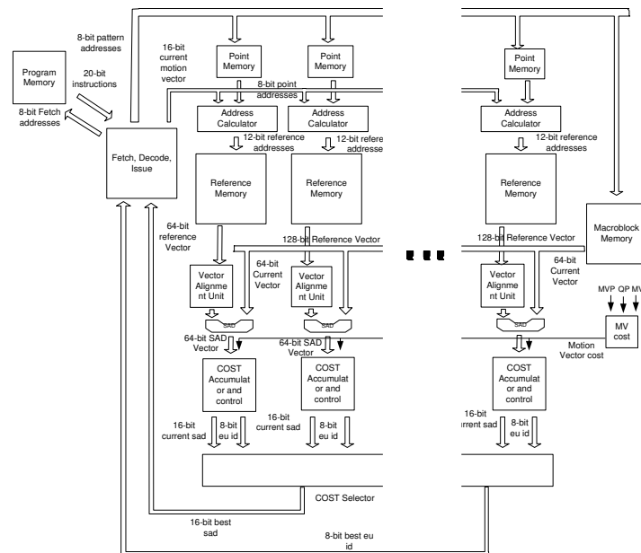
Fig. 1 Reconfigurable motion estimation processor
