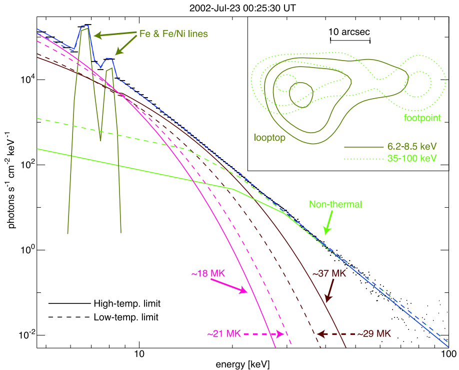
Fig. 2 Photon flux spectra ( black ) during the peak of the pre-impulsive phase of SOL2002-07-23 ( \sim 00:25:30 UT), with two acceptable model fits showing the upper ( solid ) and lower ( dashed ) temperature limits of the super-hot lines component ( brick ), as constrained by the Fe and Fe/Ni lines ( olive ). Cool isothermal ( magenta ) and non-thermal ( green ) components are also required. ( Inset ) 30%, 50%, and 90% contours of 6.2–8.5 keV ( black solid ) and 35–100 keV ( red dotted ) images at the same time. The peak non-thermal emission appears to be above the thermal looptop; the faint footpoint contains only \sim 16% of the total non-thermal flux within the 50% contour (from Caspi and Lin 2010)
