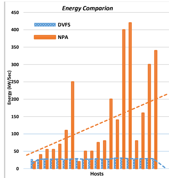
Figure 5: Consumption in a Data Center
