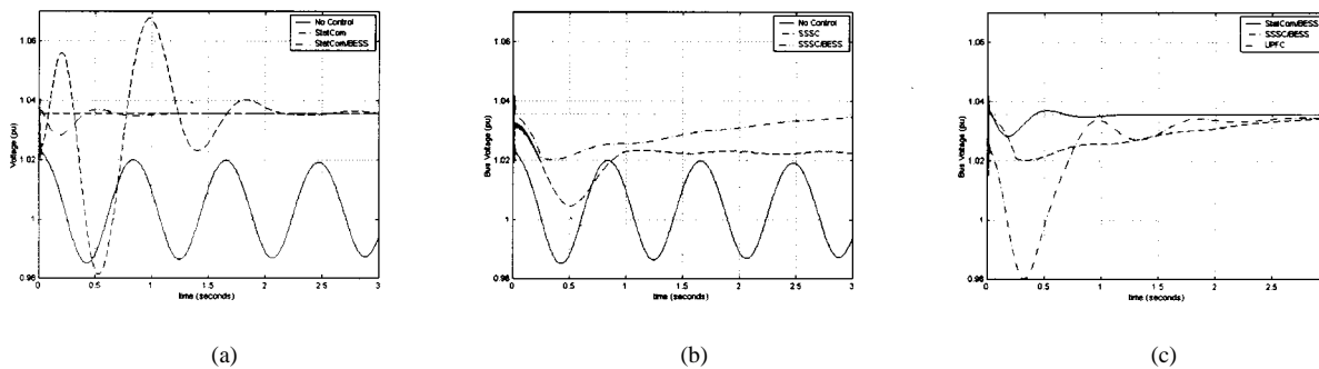
Fig. 12. Voltage at area 2 bus (6). (a) StatCom versus StatCom/BESS. (b) SSSC versus SSSC/BESS. (c) StatCom/BESS versus SSSC/BESS versus UPFC.
