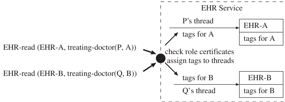
Fig. 3. Isolated threads can access different data
