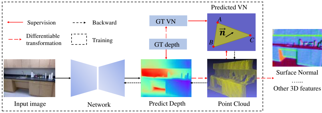
Figure 2 – Illustration of the pipeline of our method. An encoder-decoder network is employed to predict the depth, from which the point cloud can be reconstructed. A pixel-wise depth supervision is firstly enforced on the predicted depth, while a geometric supervision, virtual normal constraint, is enforced in 3D space. With the well trained model, other 3D features, such as the surface normal, can be directly recovered from the reconstructed 3D point cloud in the inference.
