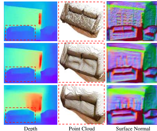
Figure 1 – Example results of ground truth (the first row), our method (the second row) and Hu et al. [21] (the third row). By enforcing the geometric constraints of virtual normals, our reconstructed 3D point cloud can represent better shape of sofa (see the left part) and the recovered surface normal has much less errors (see green parts) even though the absolute relative error (rel) of our predicted depth is only slightly better than Hu et al. (0.108 vs. 0.115).
