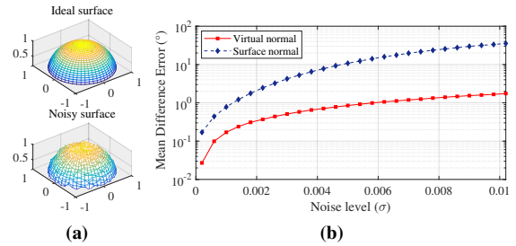
Figure 5 – Robustness of virtual normal and surface normal against data noise. (a) The ideal surface and noisy surface. (b) The Mean Difference Error (Mean) is applied to evaluate the robustness of virtual normal and surface normal against different noise level. Our proposed virtual normal is more robust.
