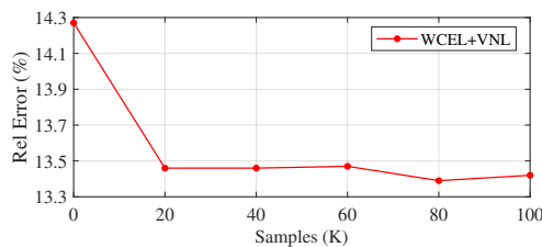
Figure 8 – Illustration of the impact of the samples size. The more samples will promote the performance.
