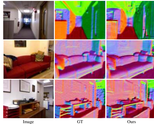
Figure 10 – Recovered surface normal from 3D point cloud. According to the visual effect, the surface normal is in high-quality in planes (1st row) and the complicated curved surface (2nd and last row).
