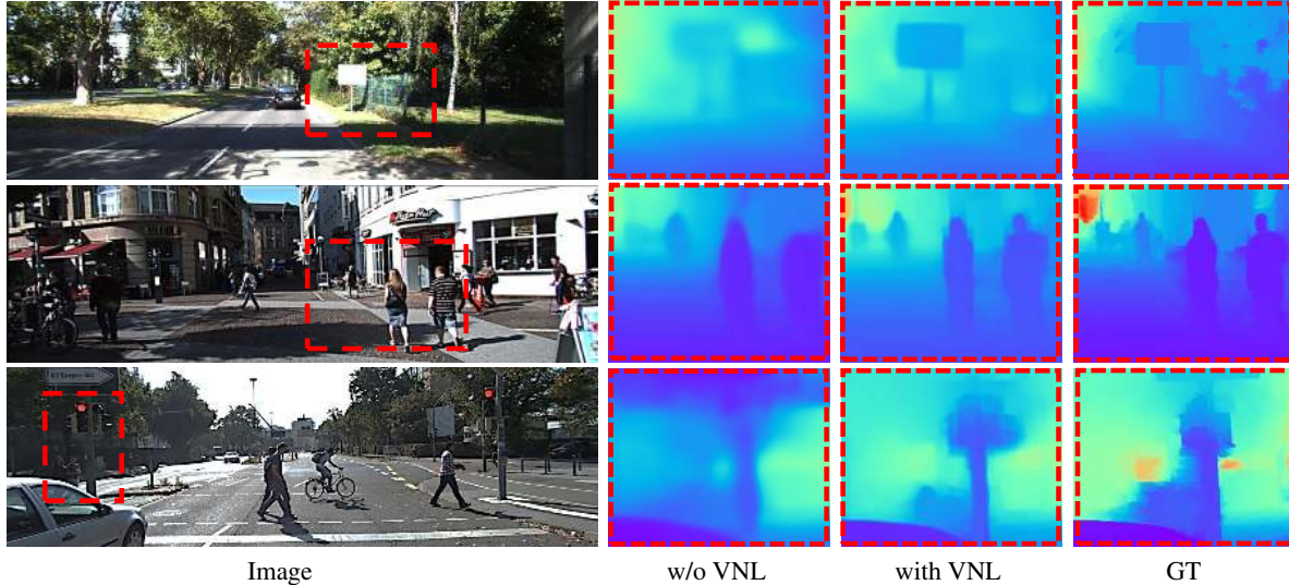
Figure 7 – Depth maps in the red dashed boxes with sign, pedestrian and traffic lights are zoomed in. One can see that with the help of virtual normal, predicted depth maps in these ambiguous regions are considerably more accurate.
