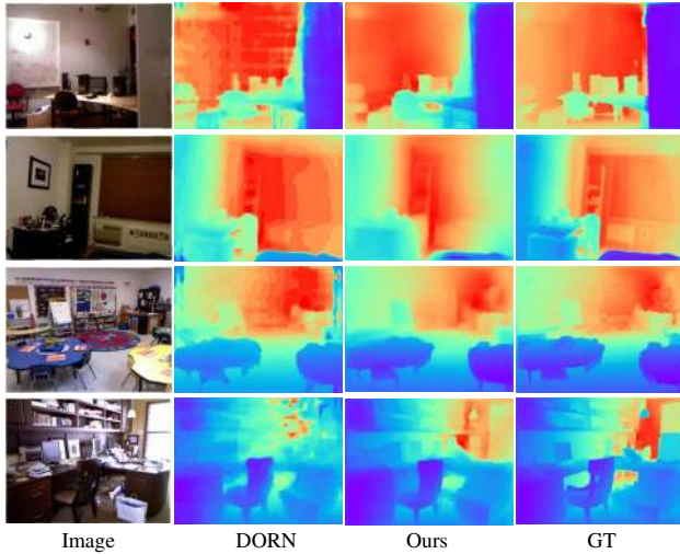
Figure 6 – Examples of predicted depth maps by our method and the state-of-the-art DORN on NYUD-V2. Color indicates the depth (red is far, purple is close). Our predicted depth maps have fewer errors in planes (see walls) and have high-quality details in complicated scenes (see the desk and shelf in the last row)
