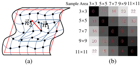
Figure 3 – Illustration of fitting point clouds to obtain the local surface normal. The directions of the surface normals is fitted with different sampling sizes on a real point cloud (a). Because of noise, the surface normals vary significantly. (b) compares the angular difference between surface normals computed with different sample sizes in Mean Difference Error. The error can vary significantly.
