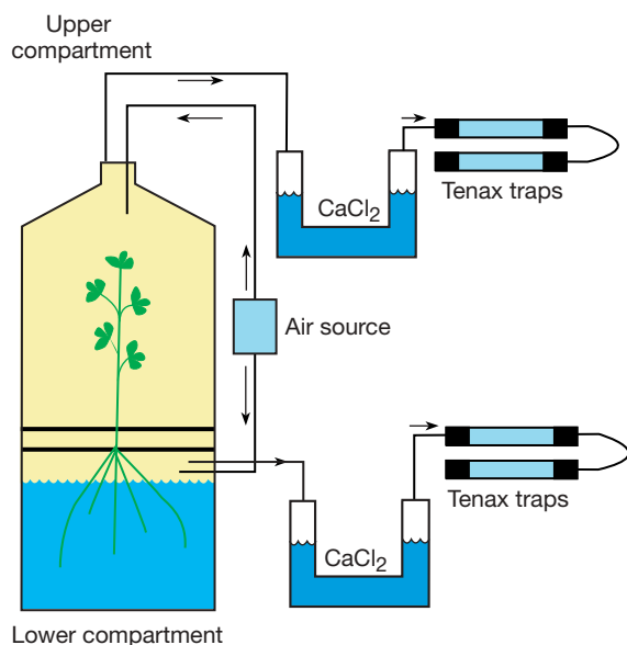
Figure 1 Schematic representation of the experimental setup for measuring toluene evapotranspiration. Yellow lupine plants are grown as hydroponics in a two-compartment glass cuvette system. Continuous airflow allows toluene from the gas phases from both compartments to collect on Tenax traps. A \text{CaCl}_2 -filled column was installed to prevent condensation of water in the Tenax traps. Tenax traps were cooled with dry ice to optimize adsorption capacities.
