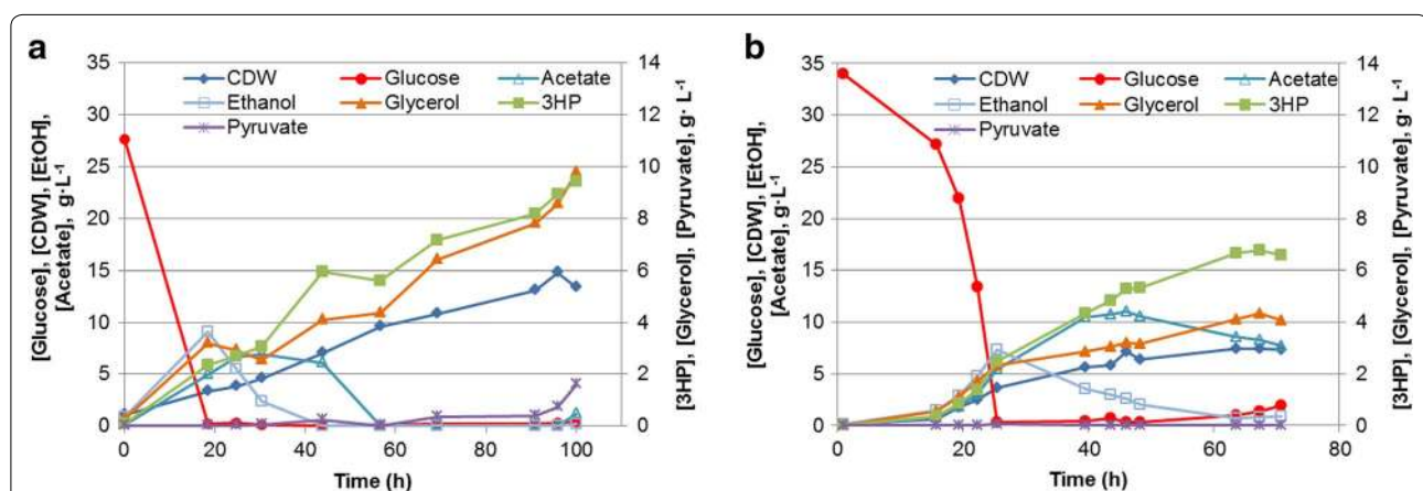
Fig. 4 Fed-batch fermentation of the best 3HP-producing strain ST687. Aerobic fed-batch fermentations were carried out under a C-limited conditions and b N/C-limited conditions. The cultivations were carried out in triplicates (Additional file 1: Fig. S4); here representative graphs are shown
