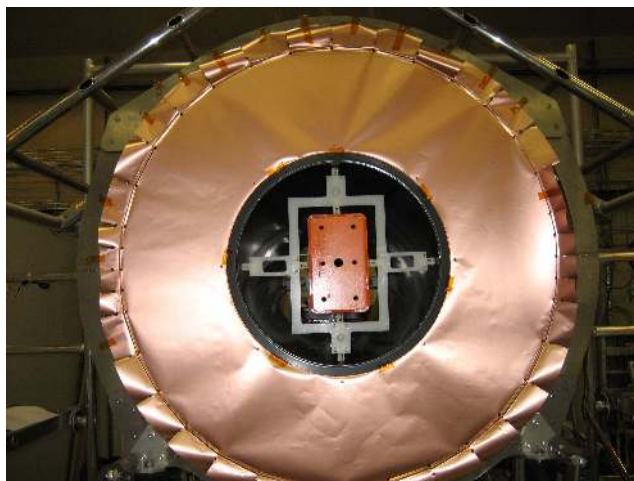
Figure 43. Front grounding-and-shielding membrane ready to be soldered to the OTE. The “V” creases in the tabs can be seen at the outer radii.
