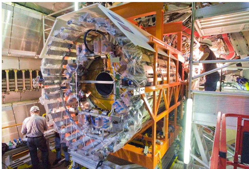
Figure 51. Installation of EC-A into ATLAS.
