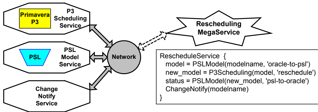
Figure 12: Rescheduling Megaservice
