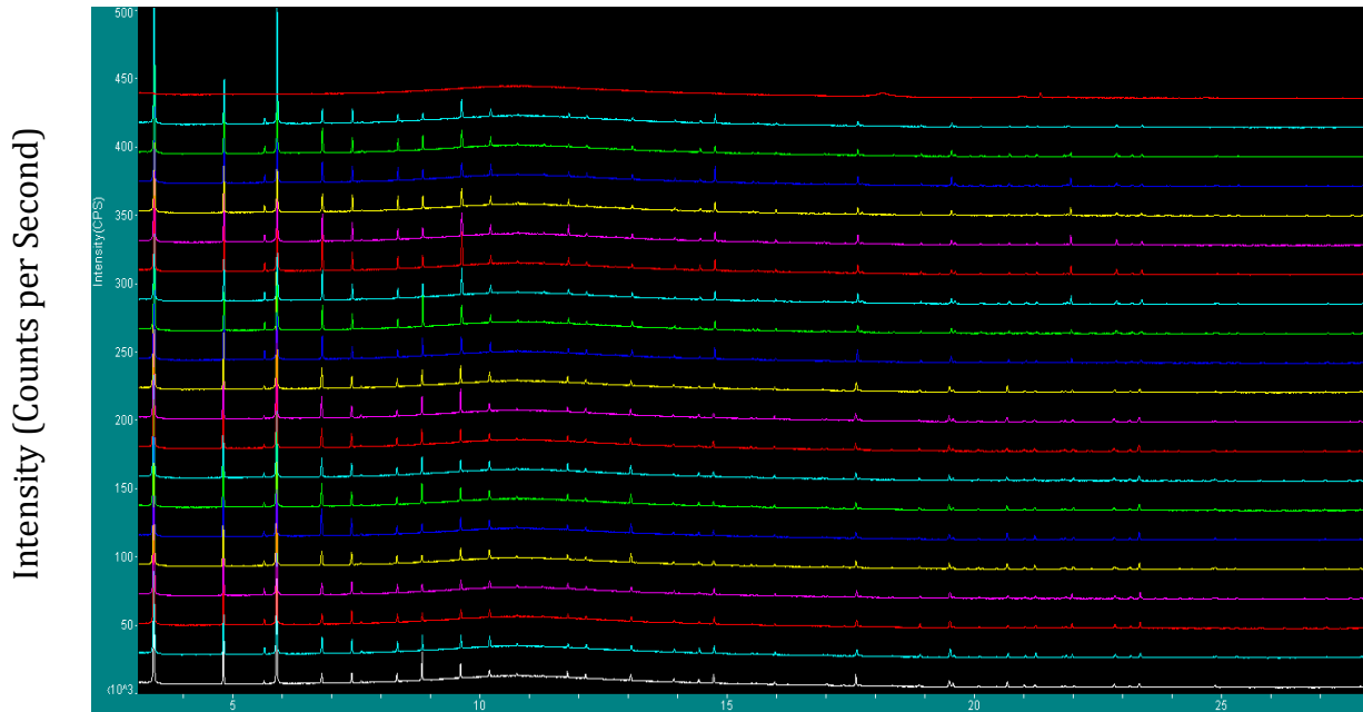
Figure 15. XRD data for Basolite showing scans from 35-350°C in flowing xenon.
