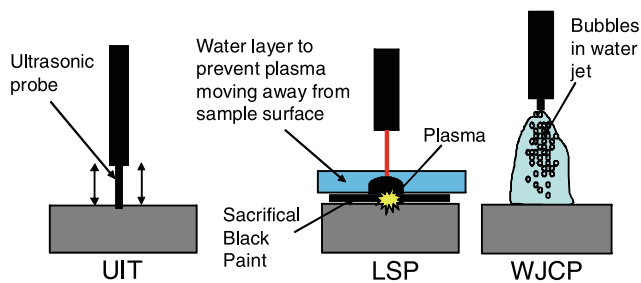
Fig. 1 Schematic description of the surface treatment process for ultrasonic impact treatment (UIT), laser shock peening (LSP), and water jet cavitation peening (WJCP)
