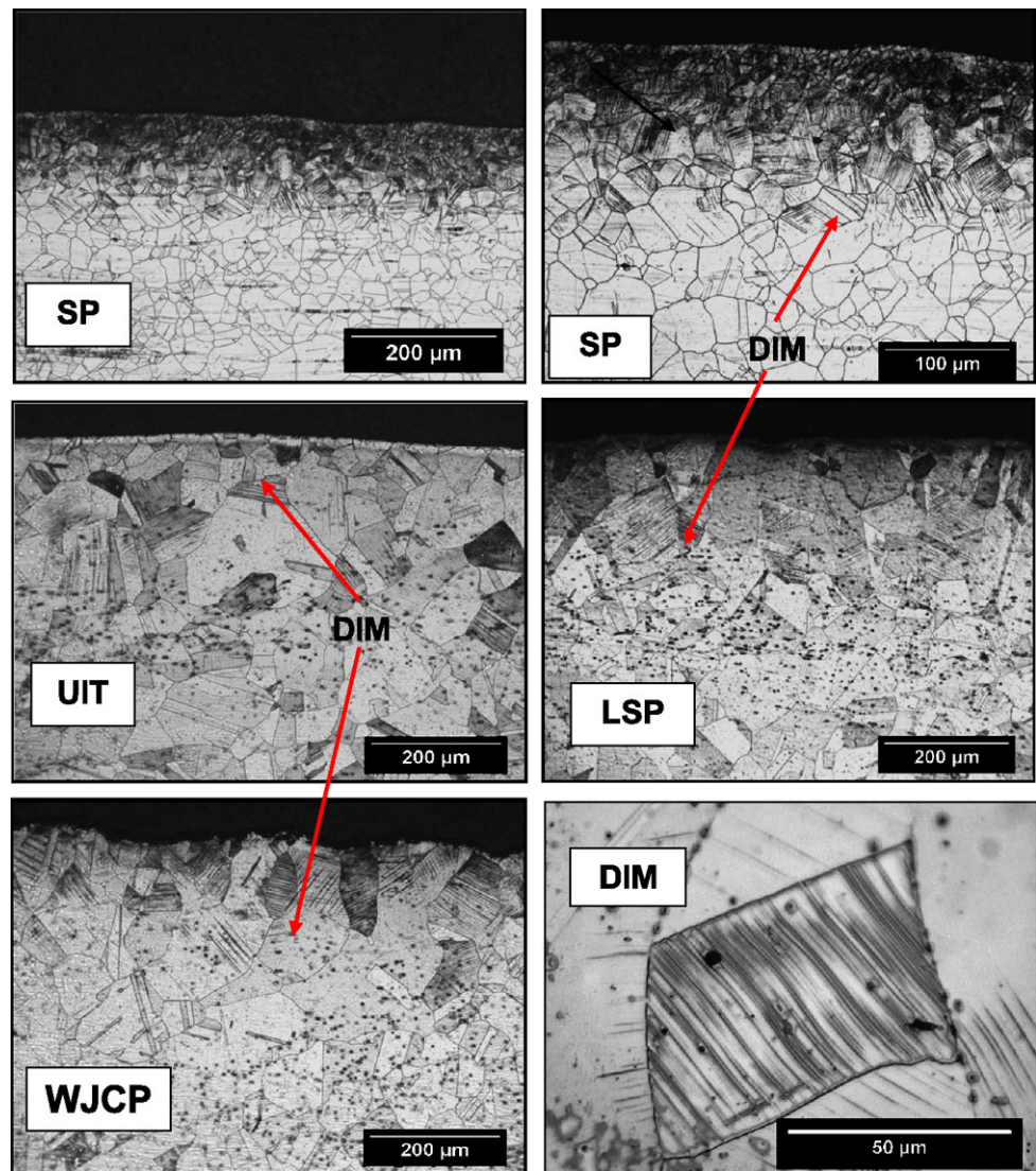
Fig. 3 Cross-sectional micrographs of the peened samples exhibiting deformation induced martensite
