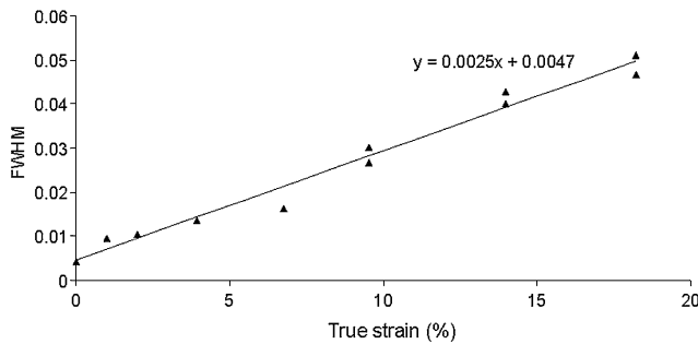
Fig. 5 Calibration plot of FWHM of the 311 crystal reflection versus true strain generated by uniaxial tensile loading
