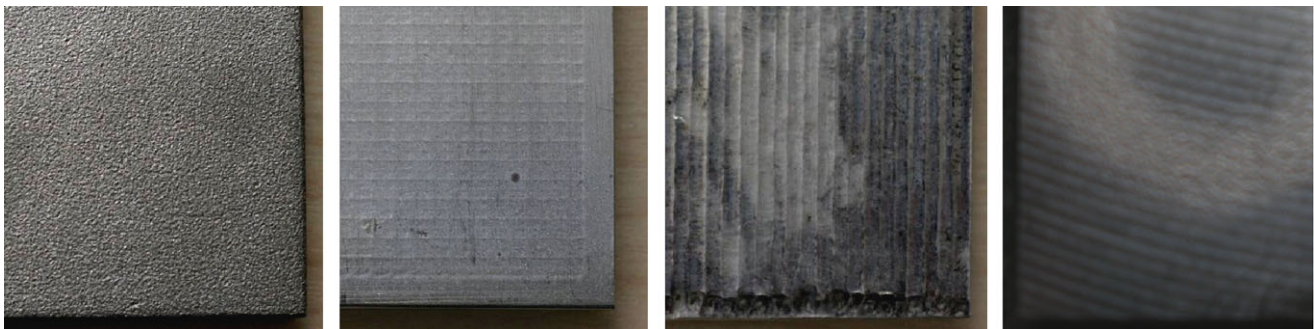
Fig. 2 Photographs of peened surface for (from left to right) SP, LSP, UIT and WJCP. The area displayed in each case is approximately 25 \times 25 mm
