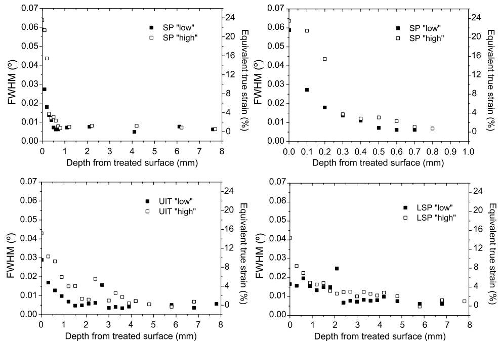
Fig. 6 The variation in diffraction peak full width half maximum measured for the (311) reflection measured on ID31 at the ESRF as a function of depth from the treated surface. The right-hand axis also denotes the equivalent plastic strain, as inferred from the calibration curve shown in Fig. 5
