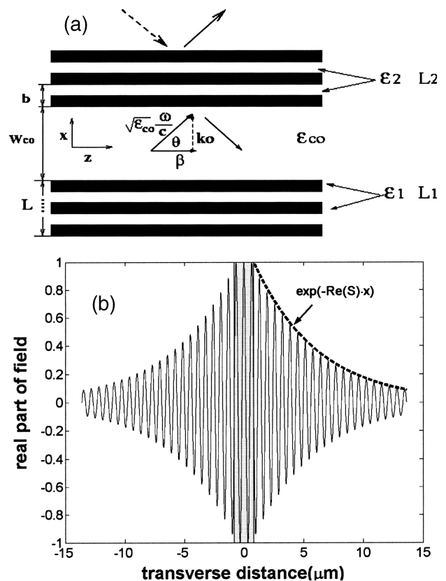
Fig. 1. (a) Schematic of a TBR waveguide. (b) Transverse field distribution of a guided TBR mode. Shaded central region, waveguide core; dashed curves, exponential decay of the form \exp[-\text{Re}(S)|x|] .
