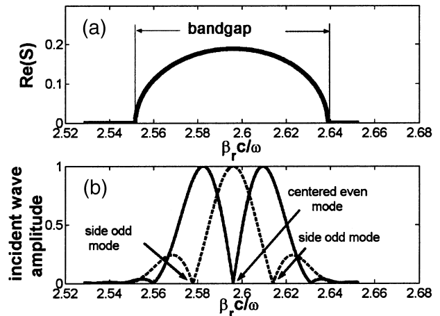
Fig. 2. (a) \text{Re}(S) as a function of effective index \beta_r c / \omega . A confined mode in a TBR waveguide is possible only in the bandgap region, with \text{Re}(S) > 0 . (b) Amplitude of the incident wave [dashed arrow in Fig. 1(a)] as a function of effective index. Solid curve, solutions with even symmetry; dashed curve, solutions of odd symmetry. Within the bandgap, at each zero-value point, Eq. (1) is satisfied, which indicates the existence of a guided TBR mode. Here we use \beta_1 = 0 , \varepsilon_{co} = \varepsilon_2 = 12.25 , W_{co} = 49.85 \mu\text{m} , and L = 32 \mu\text{m} .
