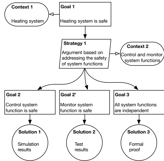
Fig. 3. Example of a GSN assurance argument
