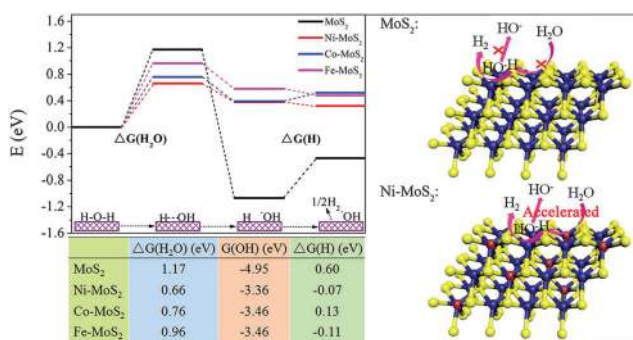
Fig. 1 The results of the DFT calculations and the corresponding mechanisms of the electrocatalytic HER on the surfaces of different catalysts under alkaline conditions. \Delta G(\text{H}_2\text{O}) and \Delta G(\text{H}) are the related kinetic energy barriers for the Volmer and Tafel steps on the catalysts, respectively. G(\text{OH}) is the Gibbs free energy of the adsorbed \text{OH}^- on the surfaces of catalysts. E (eV) in the diagram represents the free energies of the different reactive stages. The yellow, blue and red spheres represent S, Mo and Ni, respectively.
