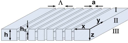
FIG. 1. (Color online) Schematics of a single slit surrounded by finite corrugations, made out of a perfect rigid body, impenetrable for airborne sound waves impinging on the structure.
