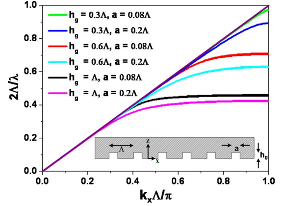
FIG. 3. (Color online) Inset shows a schematic representation of a groove grating where sound is incident in the positive z direction. Bound modes dispersion relation, Eq. (21), for different geometrical parameter a, h normalized to the period \Lambda inside the first Brillouin zone. In here the influence of the groove depth and width on the band shape is calculated.
