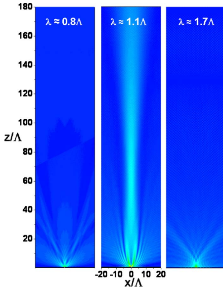
FIG. 4. (Color online) Pressure field |p(x,z)| map in the far field for a structure containing N=10 surface corrugations symmetrically around the central slit and geometries as in Fig. 2. Each panel, as indicated from left to right corresponds to wavelengths \lambda \approx 0.8\Lambda , 1.1\Lambda , and 1.7\Lambda , respectively. All field plots have been calculated with the mode matching technique described in the previous section.
