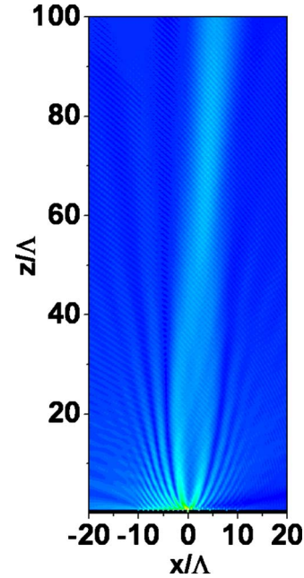
FIG. 5. (Color online) Beam steered pressure field |p(x,z)| mapping of sound through a structure with same geometry as in Fig. 2 and N=10 , though with unequal groove distances \Lambda(\sigma > 0) = 1.11\Lambda(\sigma < 0) .
