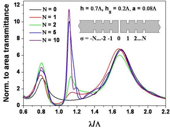
FIG. 2. (Color online) Influence on the normalized to area transmittance spectra, dependent on the numbers of surface corrugations ( N , see color legend for the value) with the geometries as specified in this figure. The acoustic plane wave is impinging normal incident on the structured system. The corrugations are symmetrically placed at the upper and lower side of the structure as the inset depicts.
