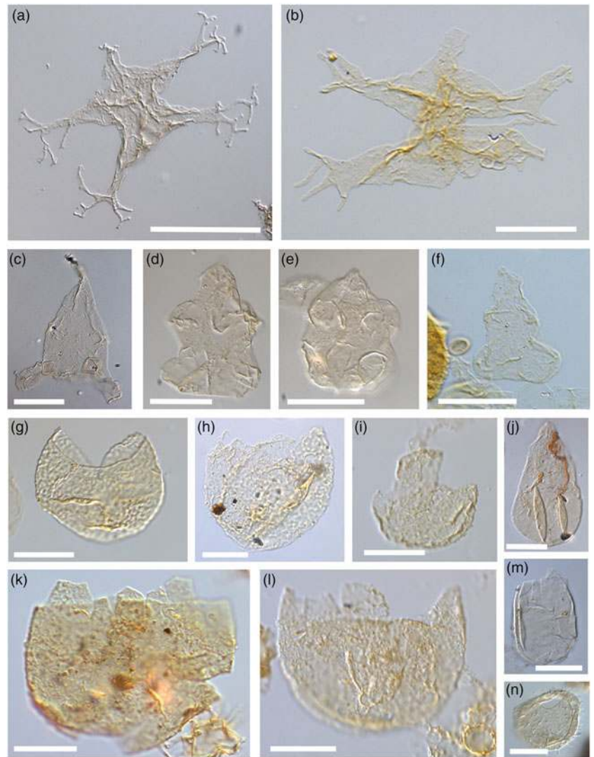
Fig. 8. Selected Pliensbachian and Toarcian dinoflagellate cyst species from Kelimyar River section S16 (all scale bars, 20 \mu m). (a) Limbicyستا bjaerkei : sample S16-07 from the Viligaensis Zone, upper Pliensbachian. Note the extremely bifurcated processes, illustrating intraspecific variability. (b) Limbicyستا bjaerkei : sample S16-80 (Kelimyar Formation), upper Toarcian. Note the generally more robust shape and processes compared with the Pliensbachian specimen. (c) Parvocysta cracens : sample S16-71 from the upper Toarcian Kelimyar Formation. (d) Susadinium scrofoides : sample S16-48 from the Commune Zone (lower Toarcian, Kelimyar Formation). (e) Parvocysta bullula : sample S16-60 from the Commune Zone (lower Toarcian, Kelimyar Formation). (f) Parvocysta tricornuta : sample S16-80 from the upper Toarcian (Kelimyar Formation). (g) Batiacasphaera sp. A: sample S16-80 from the upper Toarcian (Kelimyar Formation). (h) Batiacasphaera sp. B: sample S16-27 from the Falciferum Zone (lower Toarcian, Kelimyar Formation). (i) Dissiliodinium sp.: sample S16-30 from the Falciferum Zone (lower Toarcian, Kelimyar Formation). (j) Phallocysta eumekes : sample S16-60 from the Commune Zone (lower Toarcian, Kelimyar River). (k) Mancodinium semitabulatum : sample S16-09 from the Viligaensis Zone (Kyra Formation, upper Pliensbachian). (l) Mancodinium semitabulatum : sample S16-30 from the Falciferum Zone (lower Toarcian, Kelimyar Formation). (m) Valvaedinium aquilonium : sample S16-49 from the Commune Zone (lower Toarcian, Kelimyar Formation). (n) Valvaedinium cavum : sample S16-21 from the Falciferum Zone (lower Toarcian, Kelimyar River).
