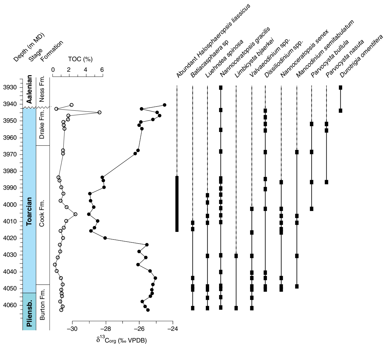
Fig. 6. Range chart and carbon isotope record for the Gullfaks 34/10-35 core.
