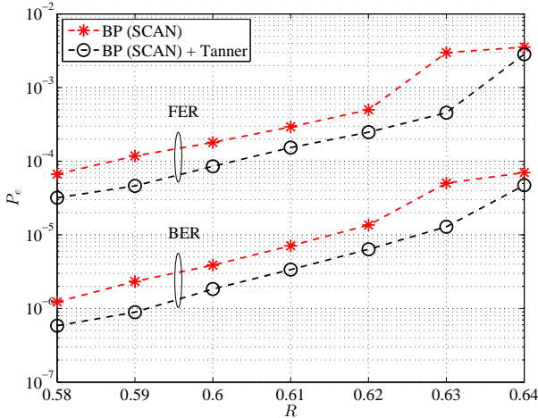
Fig. 5. BER/FER of BP SCAN over the AWGN channel at \text{SNR} = 4 dB.
