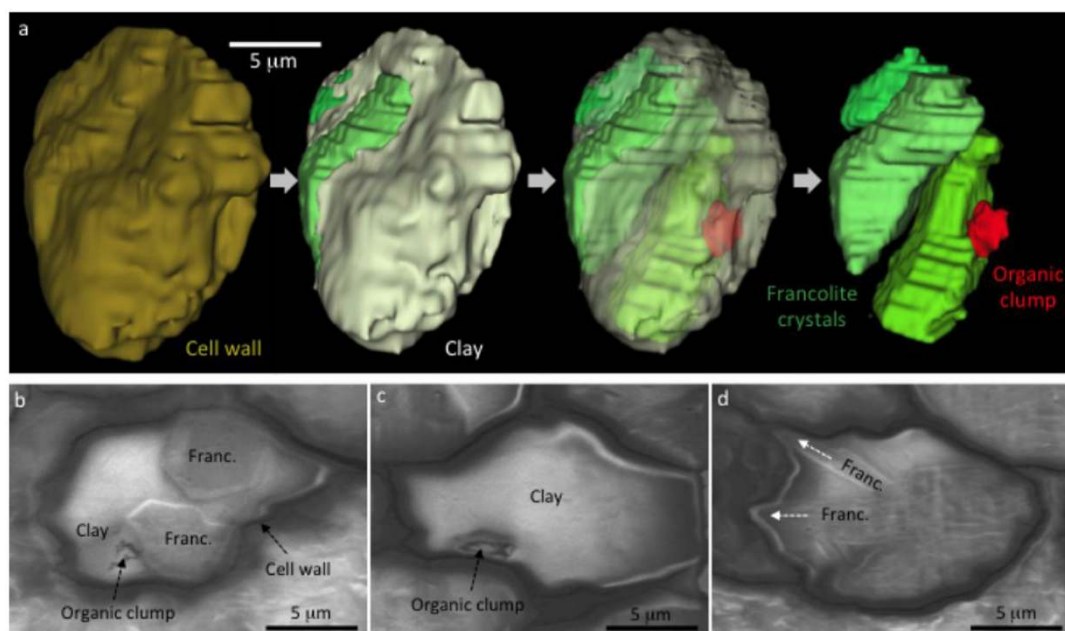
Figure 8 | Microfossil preservation quality in clay minerals. (a) 3D reconstruction of a prokaryote cell. Overview of the carbonaceous cell wall exterior is shown on the left. Next, the cell wall is removed to show the cell interior mineralized by clay (white) and three calcium phosphate (francolite) crystals (green). The clay portion is then made transparent to show that clays enclose degraded remains of putative cell contents (red). Finally (right), the clays are removed to show that the putative cell contents (organic clump) are not enclosed by francolite. (b) A single FIB-SEM slice through the microfossil reconstructed in (a), showing the 2D relationship between the cell wall, francolite, clay minerals, and the organic clump interpreted as putative cell contents. (c) A second example of a prokaryote cell with putative cell contents preserved in clay. (d) A prokaryote cell fossilized by a mixture of clay and francolite, showing how the growth of two elongate francolite crystals (arrows) caused modification of the cell wall.
