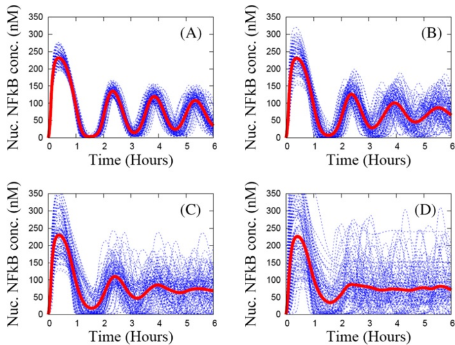
Figure 7 Dependence of the individual time-series curves (blue lines) and the statistical ensemble average (red line) of nuclear NF- \kappa B profiles for a mutant with \text{I}\kappa\text{B}\beta and \text{I}\kappa\text{B}\epsilon genes double knocked-out, on the heterogeneity factor \chi (the interval size of the uniform distribution or kinetic rate parameters). (A) \chi = 10\% ; (B) \chi = 30\% ; (C) \chi = 50\% ; (D) \chi = 70\% .
