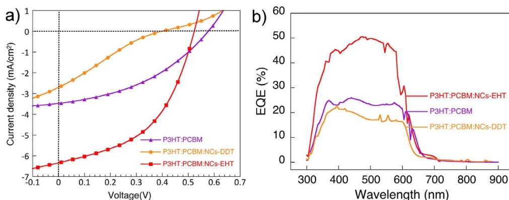
Figure 4 | (a) J(V) curves obtained under simulated solar light (AM1.5 one sun conditions) of solar cells containing ternary blends of P3HT, PCBM and DDT- or EHT-capped CuInS 2 NCs (1:1:0.5 mass ratio) after 15 min annealing at 120°C. For comparison the curve obtained with an identical solar cell containing the binary P3HT:PCBM mixture (1:1 mass ratio) is shown. (b) External quantum efficiency spectra of the different solar cells measured under identical illumination conditions.
