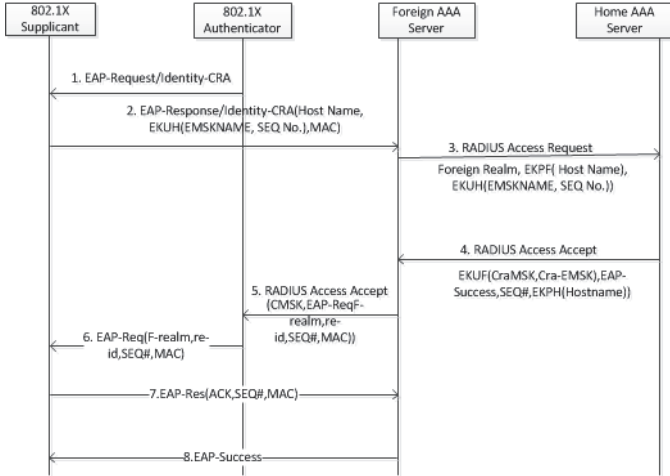
Fig. 1. Coordinated Robust Authentication (CRA) Full Authentication Protocol.
