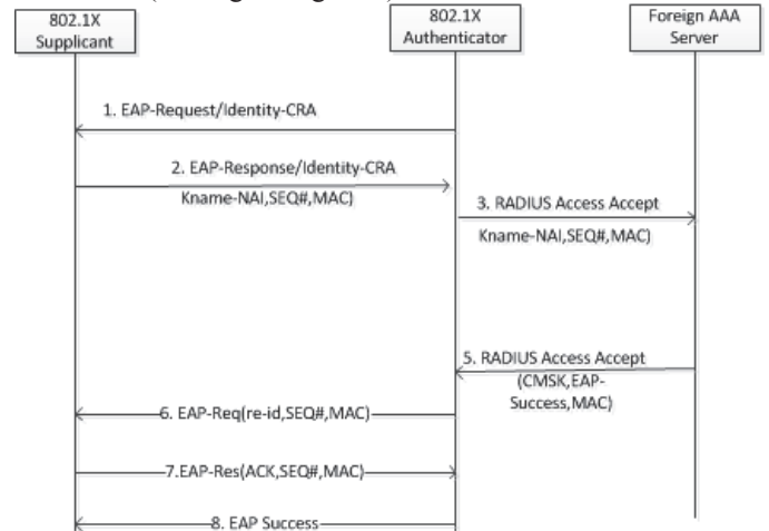
Fig. 2. EAP-CRA Re-authentication
