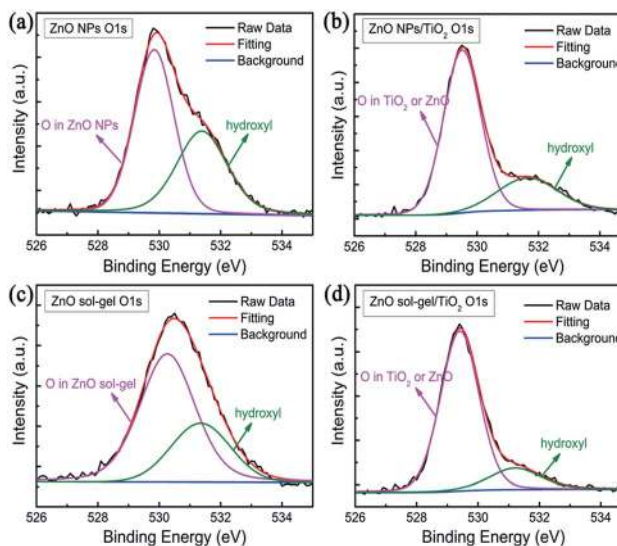
Fig. 3 XPS spectra of (a) a ZnO-NP film, (b) a ZnO NPs/TiO 2 bilayered film, (c) a ZnO sol-gel film, and (d) a ZnO sol-gel/TiO 2 bilayered film.
