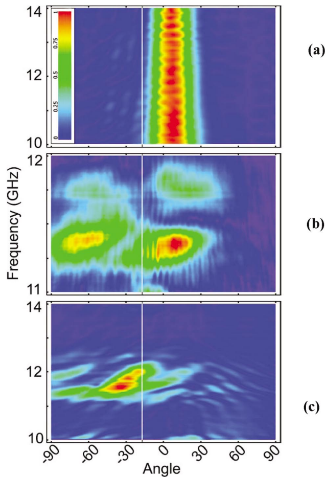
FIG. 4 (color). Map of the transmitted power as a function of frequency (vertical axis) and angle away from direct incidence (horizontal axis), for (a) a Teflon wedge with 15 mm \times 5 mm steps; (b) the Shelby et al. wedge; (c) the 2.5 mm unit-cell wedge. The vertical white lines indicate the angle of the surface normal.
