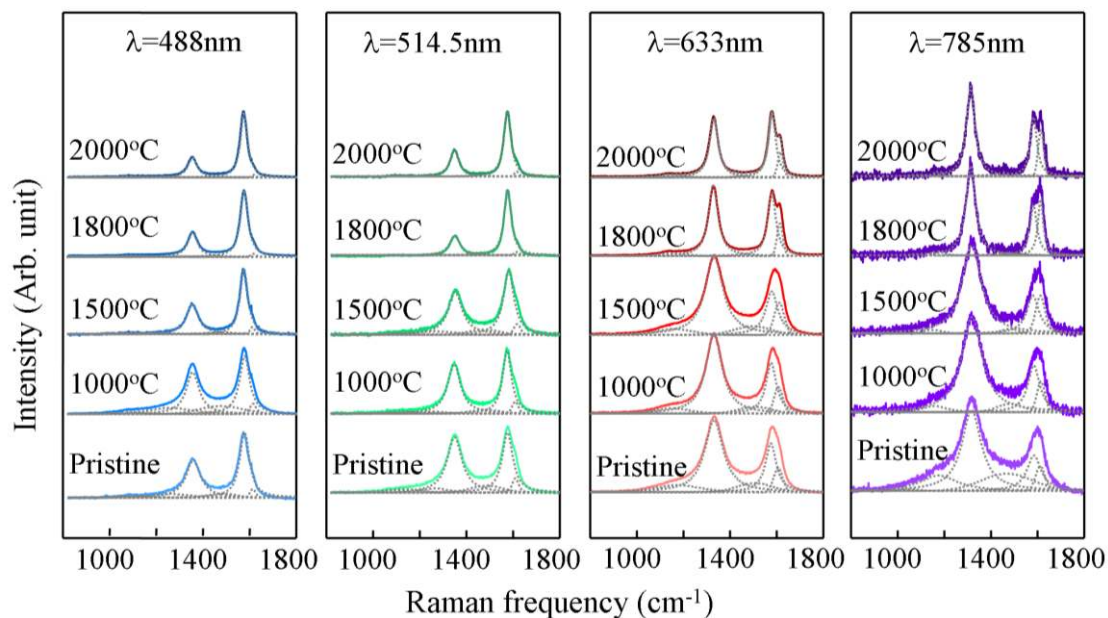
Fig. 4 Raman spectra of pristine N-doped MWNTs and thermally annealed N-doped MWNTs, in an argon atmosphere, at temperatures ranging between 1000 °C and 2000 °C, using four laser lines (488, 514.5, 633 and 785 nm).
