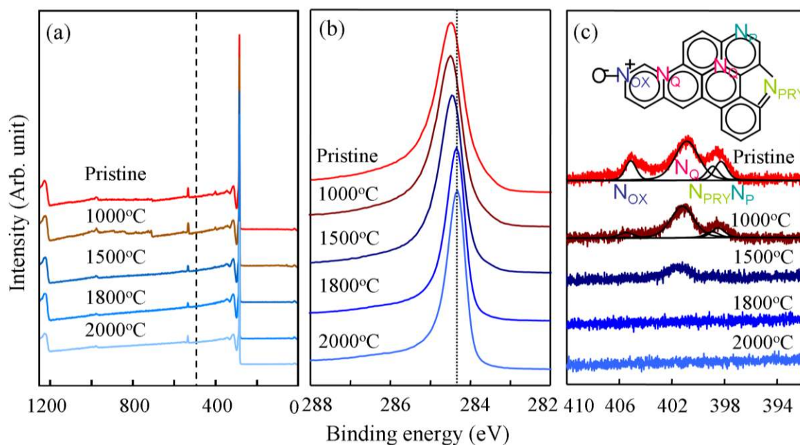
Fig. 5 XPS data of pristine N-doped MWNTs and thermally annealed N-doped MWNTs at temperatures ranging between 1000 °C and 2000 °C. (a) The wide-scan, (b) C 1s region and (c) N 1s region.
