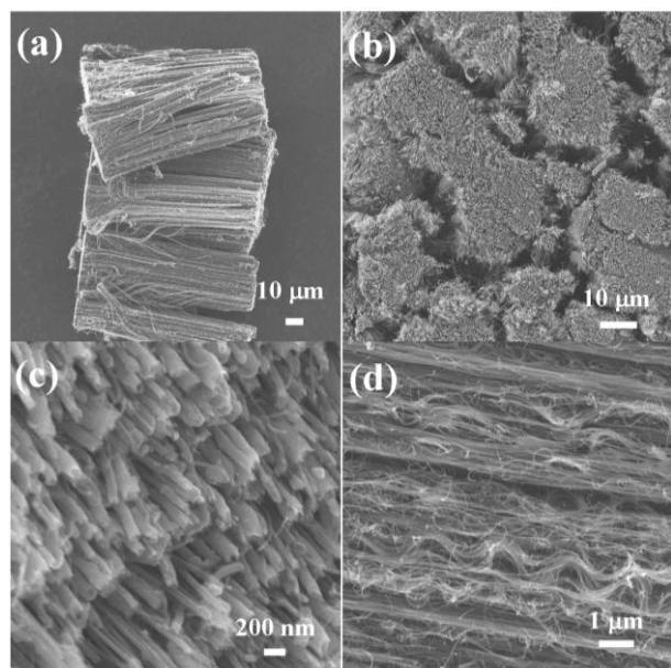
Fig. 1 (a-d) SEM images of vertically aligned N-doped MWNTs at different angles and magnifications. Note that the tube ends are opened.
