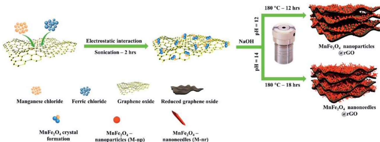
Scheme 1 Schematic illustration of hydrothermal synthesis of morphologically tuned \text{MnFe}_2\text{O}_4/\text{rGO} nanocomposites of nanoparticles and nanoneedles.
